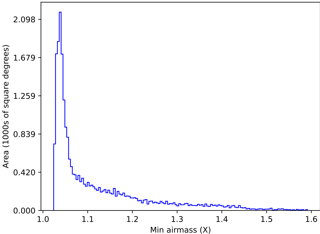
too_ignore_100_4v3.4_10yrs All sky u band: Min airmass
