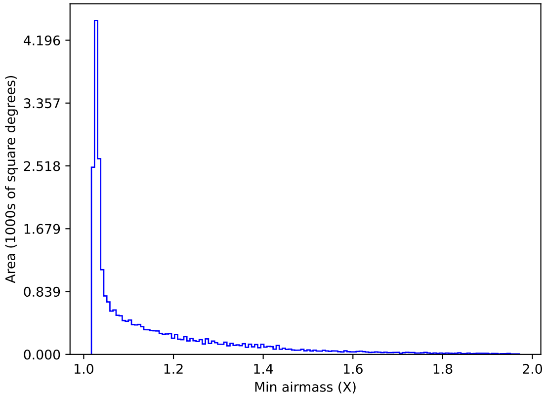
too_ignore_100_4v3.4_10yrs All sky r band: Min airmass
