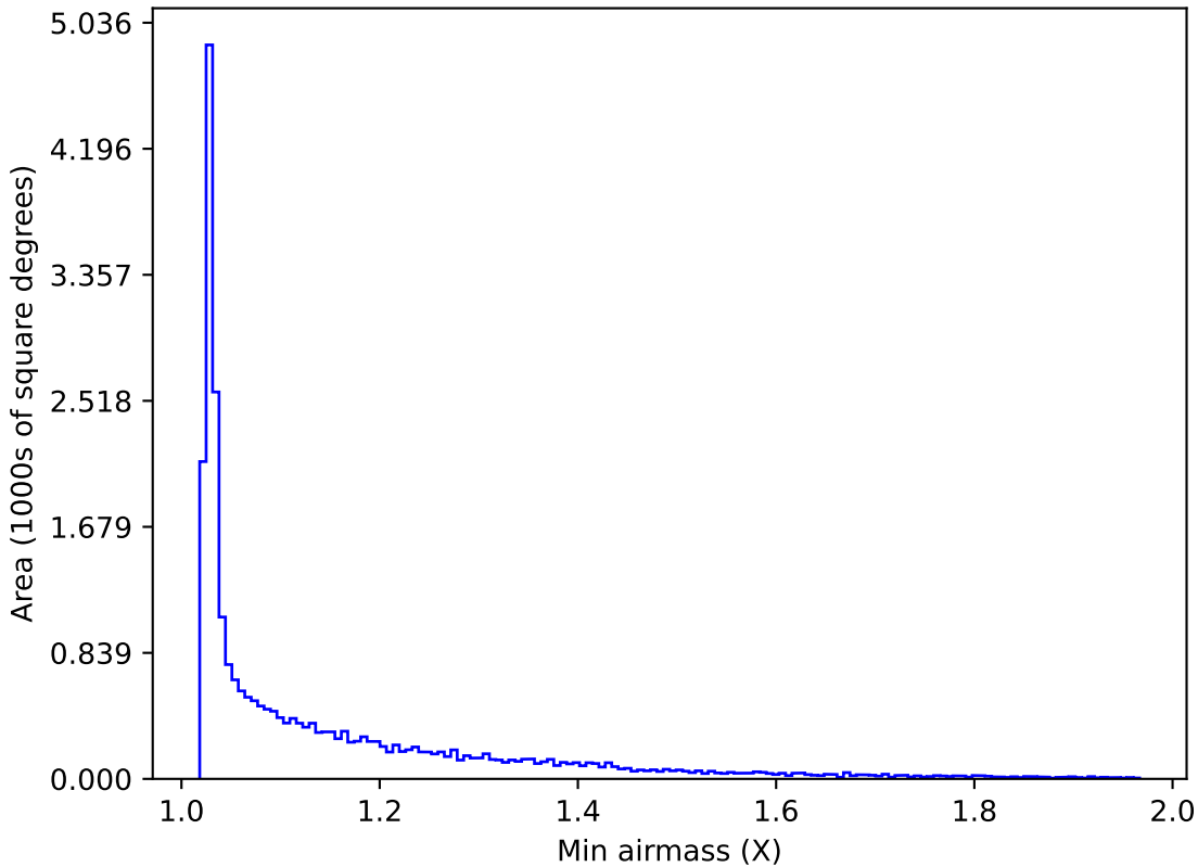
too_ignore_100_4v3.4_10yrs All sky i band: Min airmass
