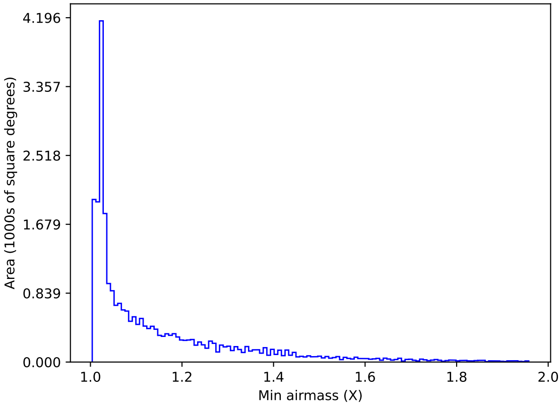
too_ignore_100_4v3.4_10yrs All sky all bands: Min airmass
