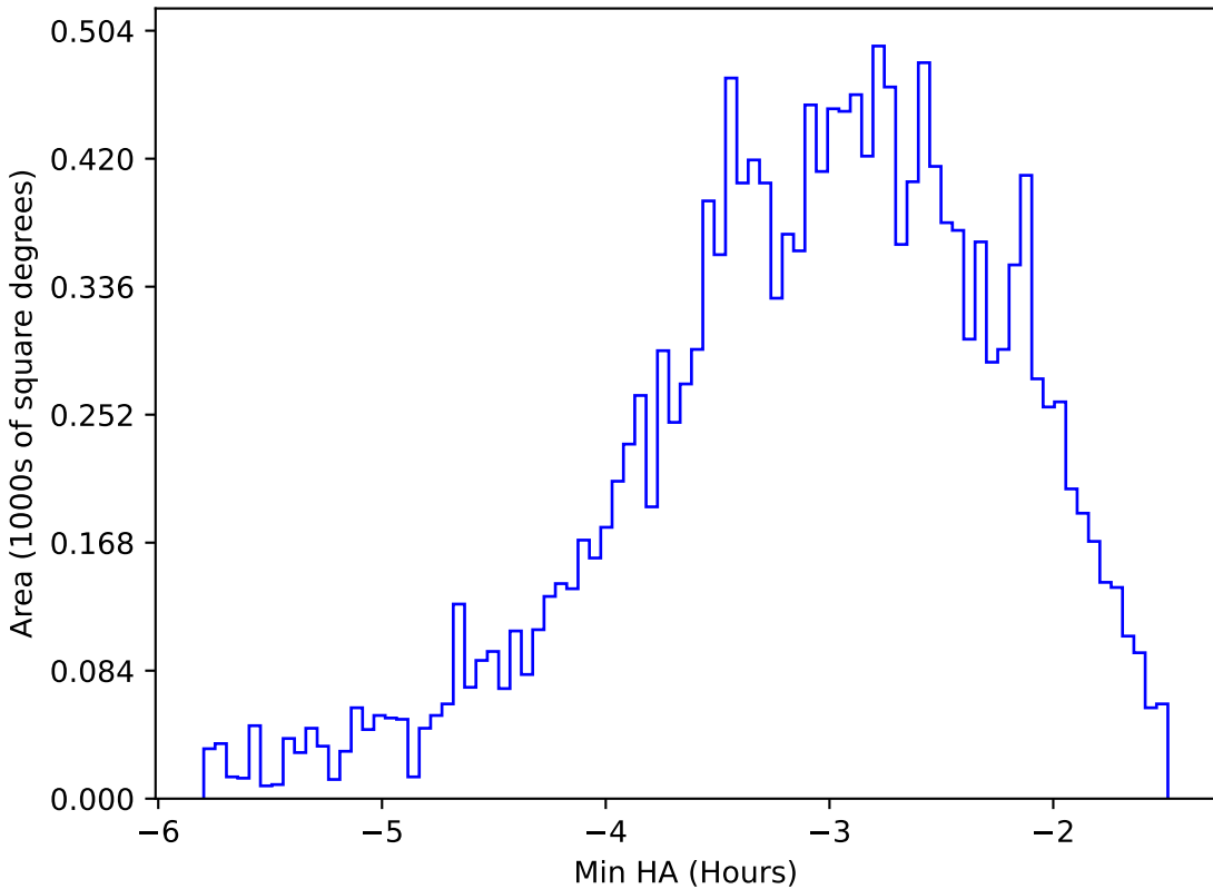
too_ignore_100_4v3.4_10yrs WFD u band: Min HA
