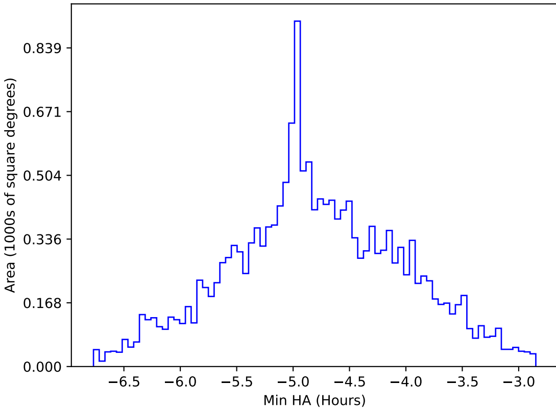
too_ignore_100_4v3.4_10yrs WFD all bands: Min HA
