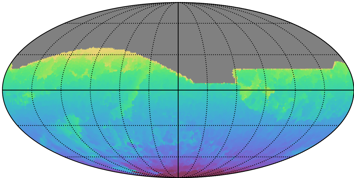
too_ignore_100_4v3.4_10yrs All sky all bands: Min HA
