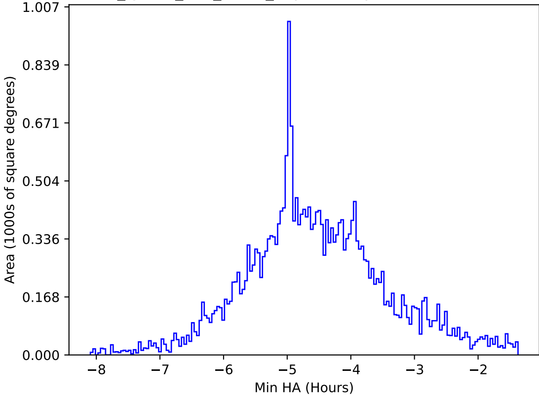
too_ignore_100_4v3.4_10yrs All sky all bands: Min HA
