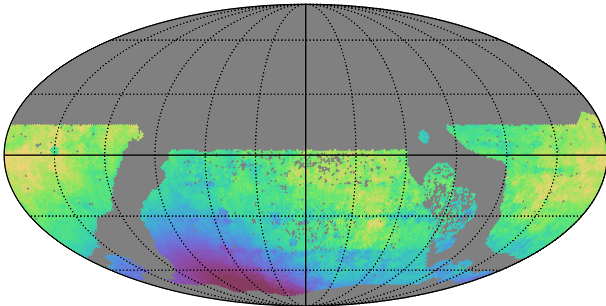
too_ignore_100_4v3.4_10yrs WFD z band: Median solarElong
