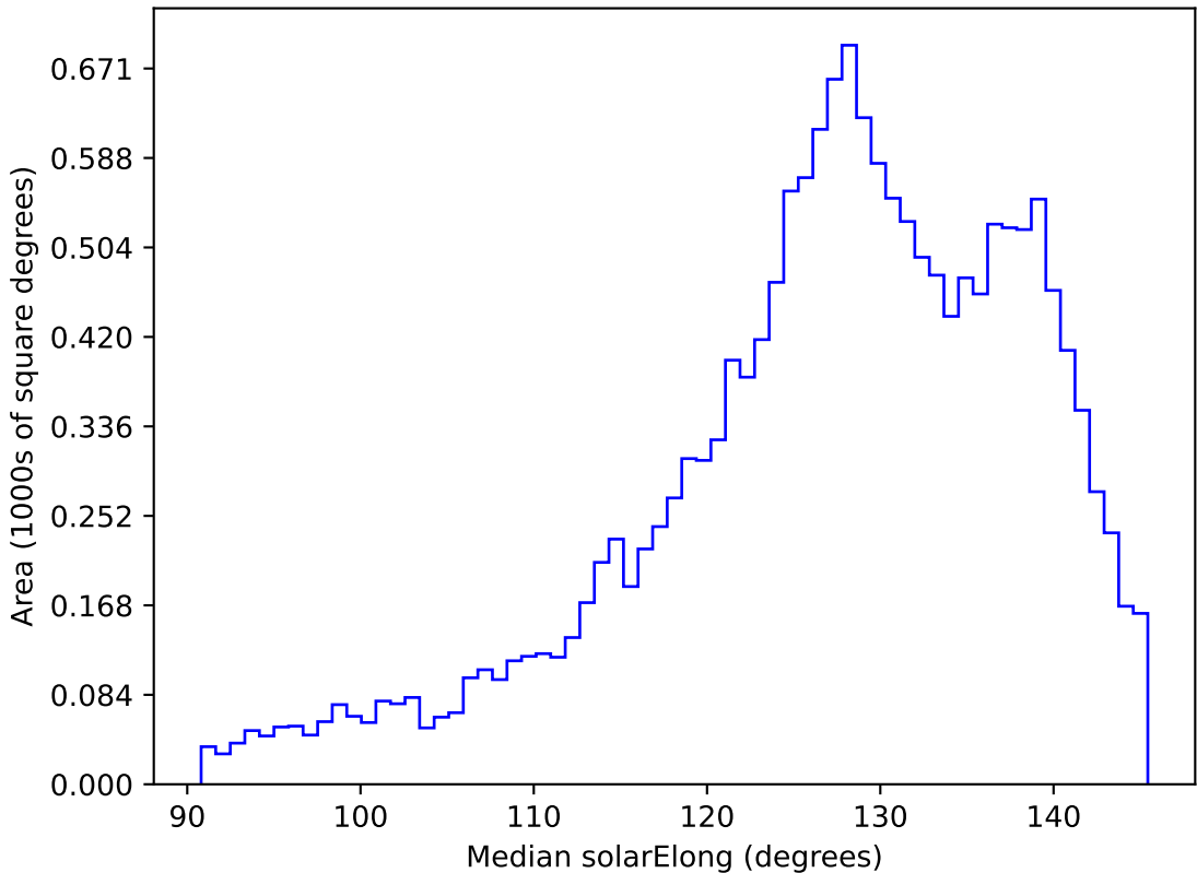
too_ignore_100_4v3.4_10yrs WFD z band: Median solarElong
