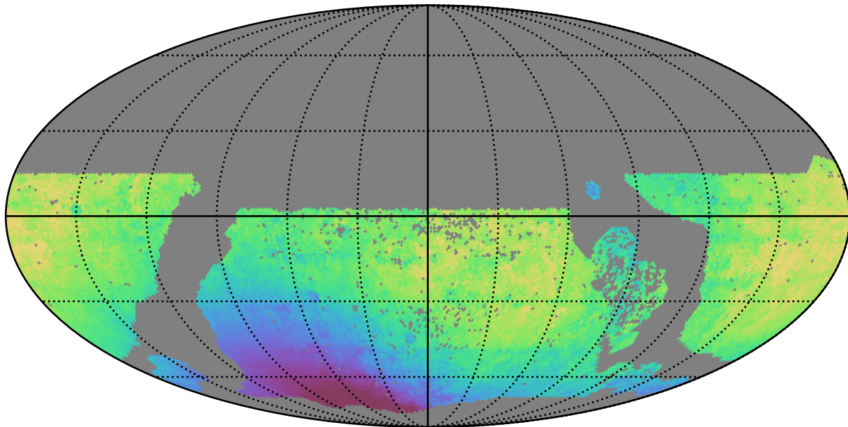
too_ignore_100_4v3.4_10yrs WFD y band: Median solarElong
