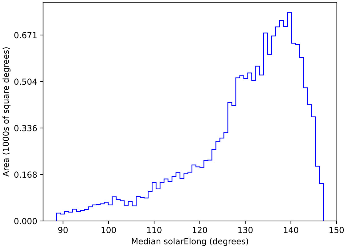
too_ignore_100_4v3.4_10yrs WFD y band: Median solarElong
