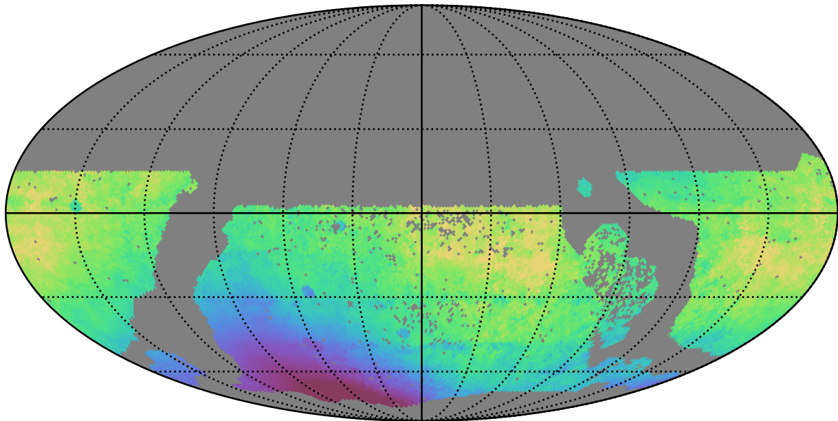
too_ignore_100_4v3.4_10yrs WFD i band: Median solarElong
