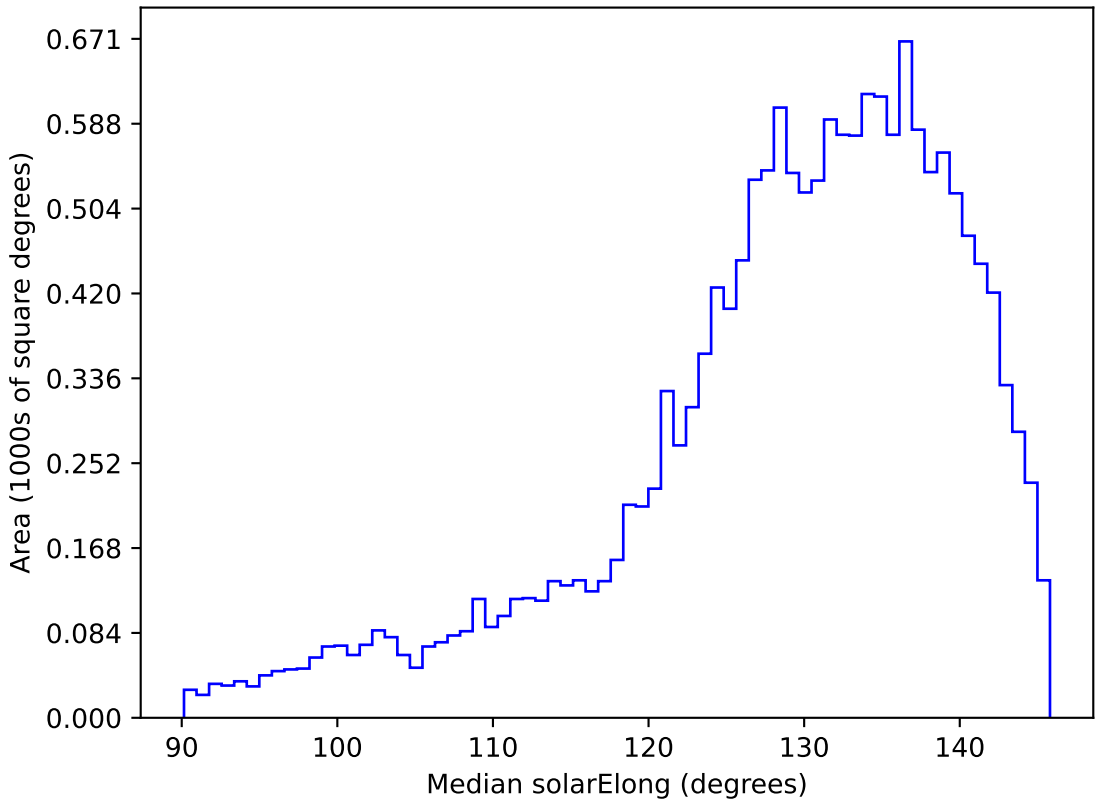
too_ignore_100_4v3.4_10yrs WFD i band: Median solarElong
