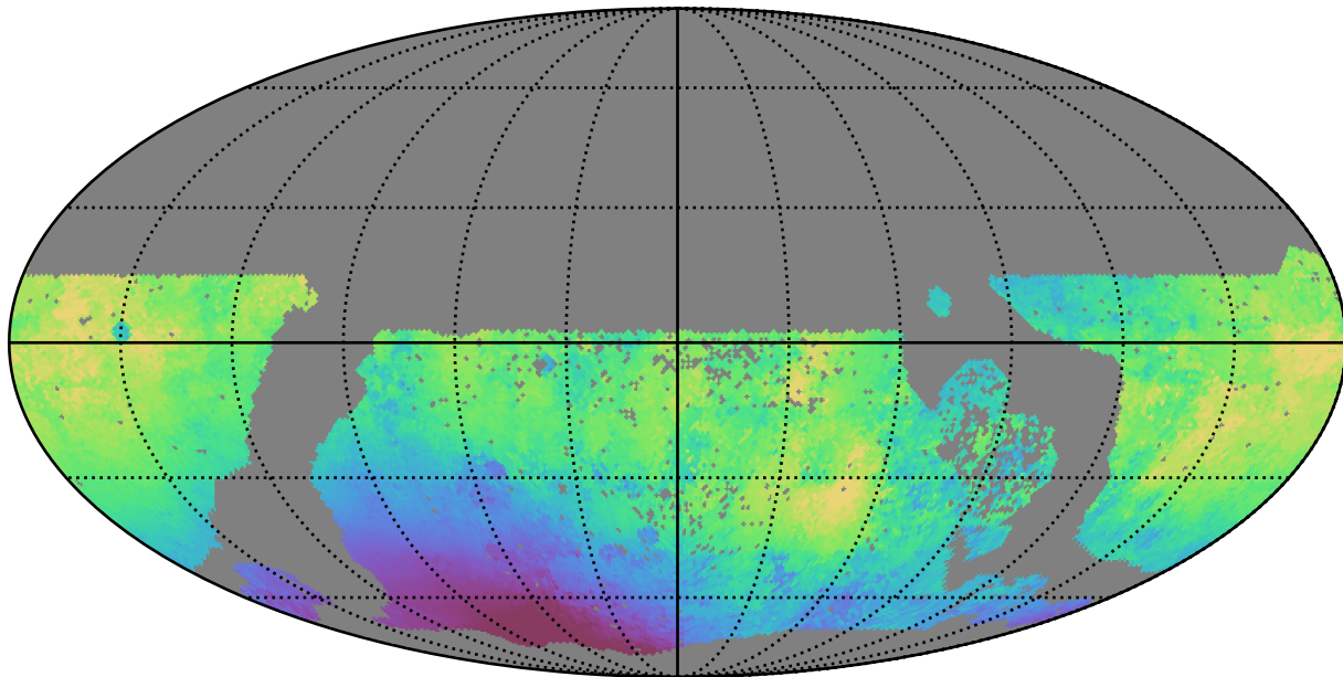
too_ignore_100_4v3.4_10yrs WFD g band: Median solarElong
