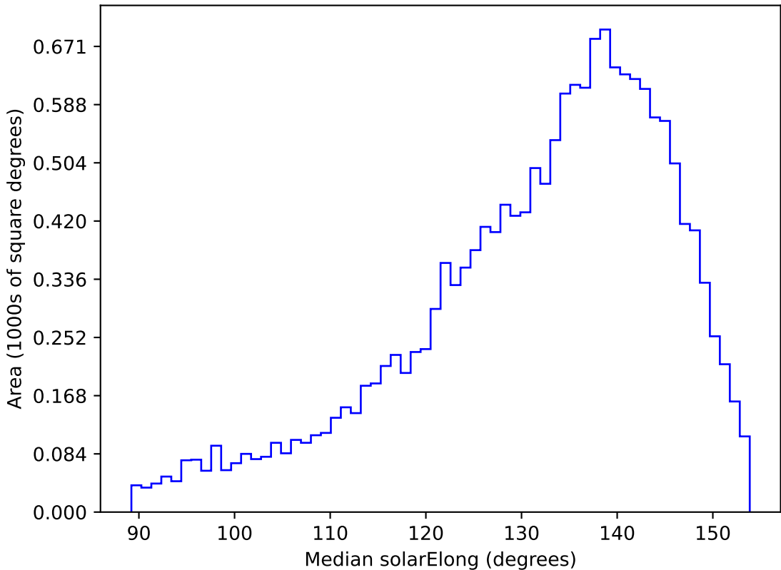
too_ignore_100_4v3.4_10yrs WFD g band: Median solarElong
