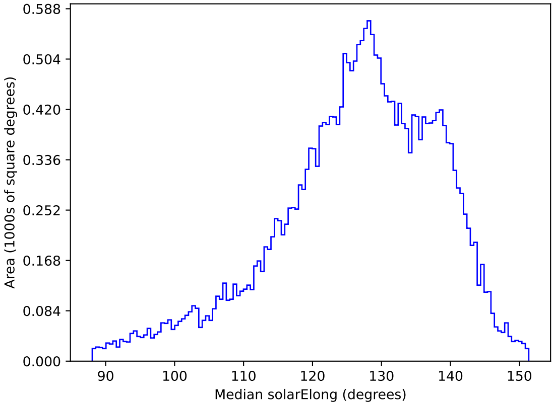
too_ignore_100_4v3.4_10yrs All sky z band: Median solarElong
