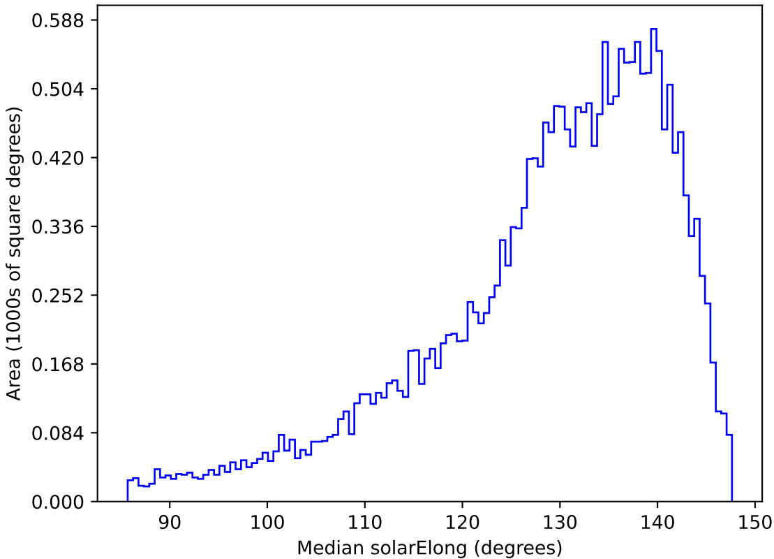
too_ignore_100_4v3.4_10yrs All sky y band: Median solarElong
