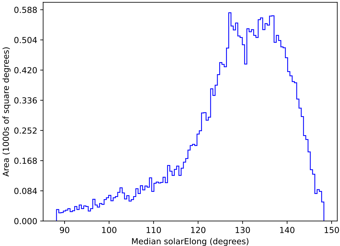
too_ignore_100_4v3.4_10yrs All sky i band: Median solarElong
