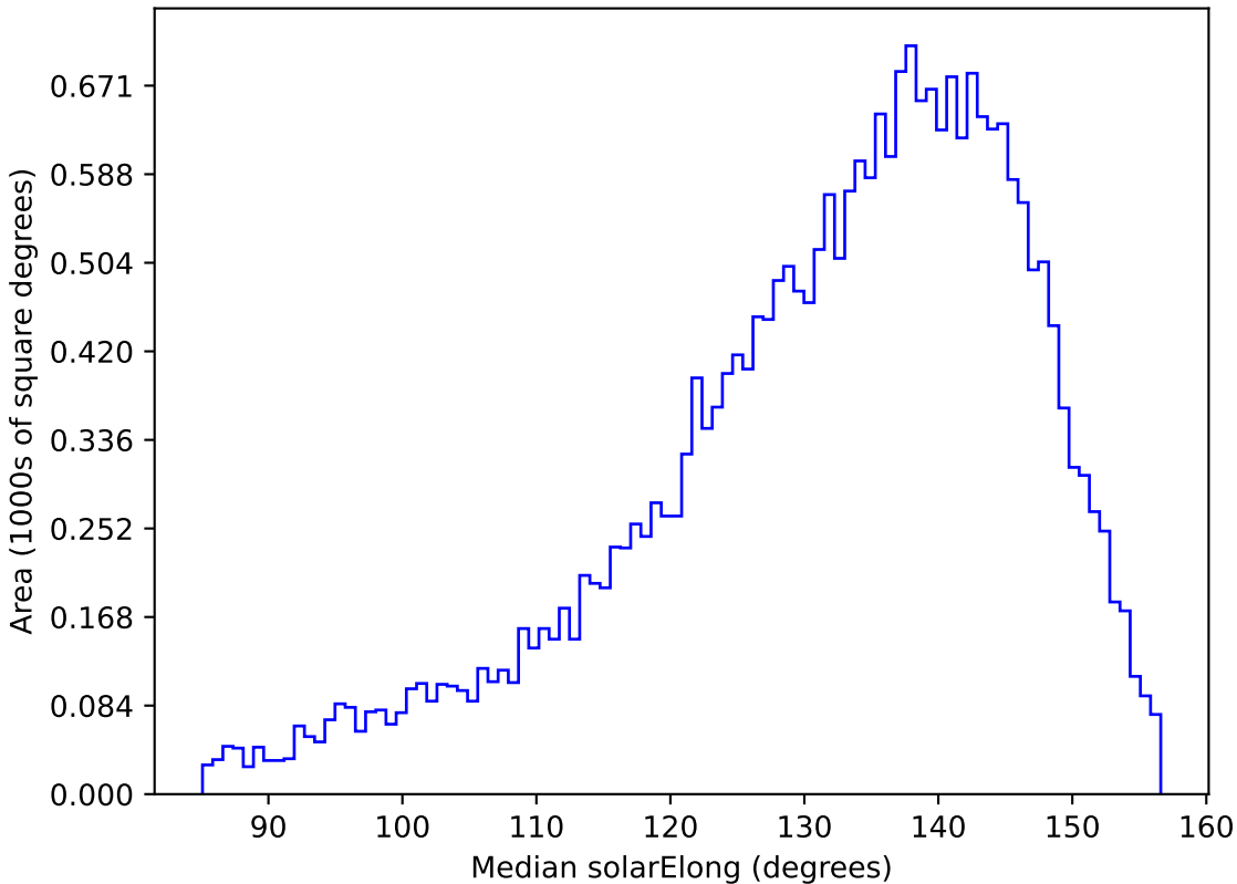
too_ignore_100_4v3.4_10yrs All sky g band: Median solarElong
