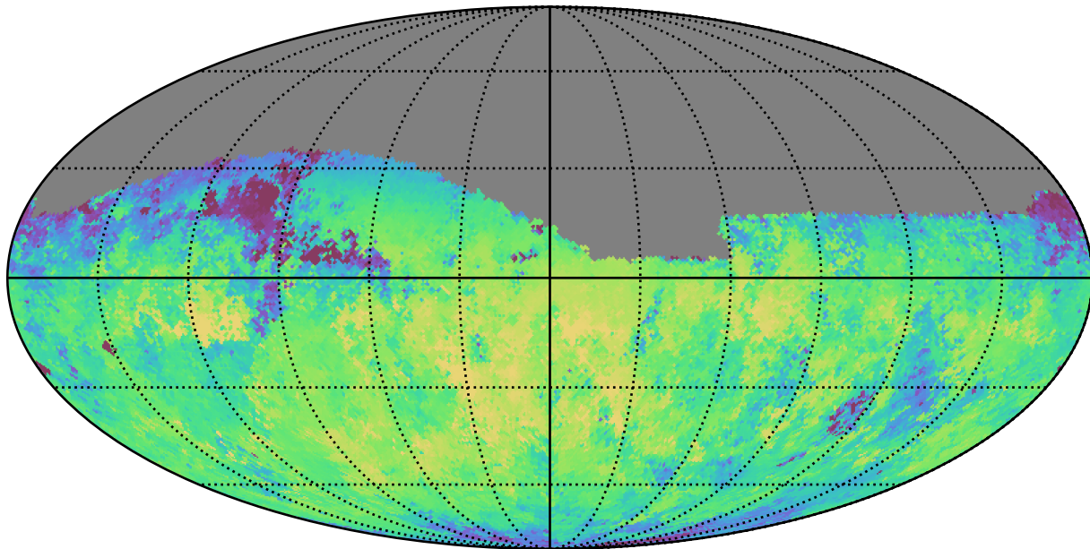
too_ignore_100_4v3.4_10yrs Yr 1 z band: Median skyBrightness
