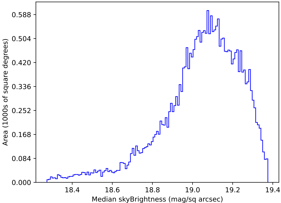
too_ignore_100_4v3.4_10yrs Yr 1 z band: Median skyBrightness
