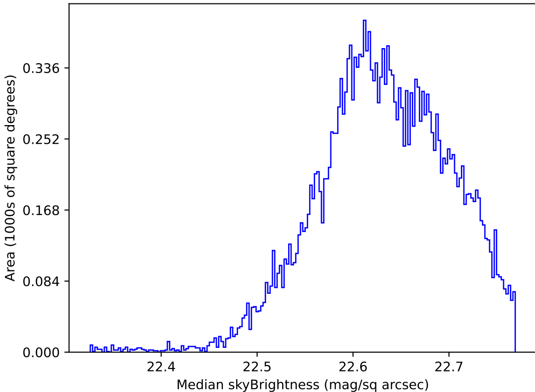
too_ignore_100_4v3.4_10yrs Yr 1 u band: Median skyBrightness
