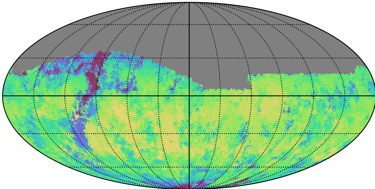
too_ignore_100_4v3.4_10yrs Yr 1 i band: Median skyBrightness
