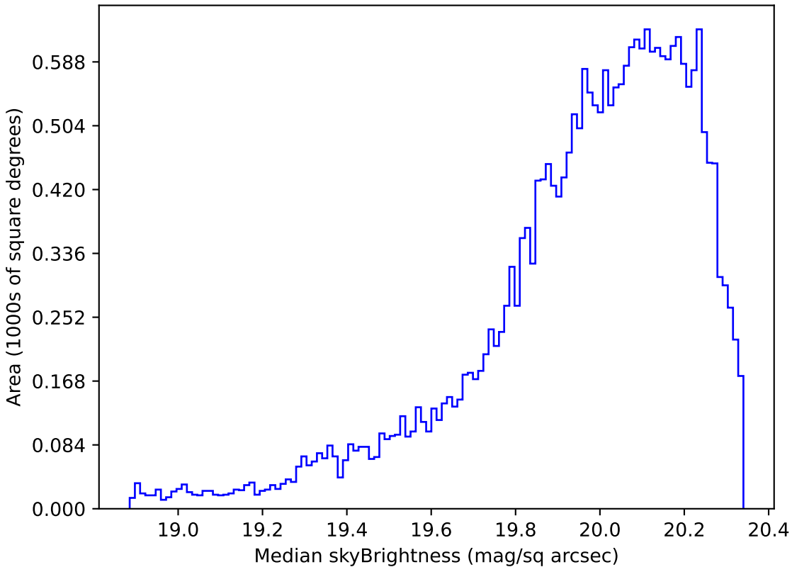
too_ignore_100_4v3.4_10yrs Yr 1 i band: Median skyBrightness
