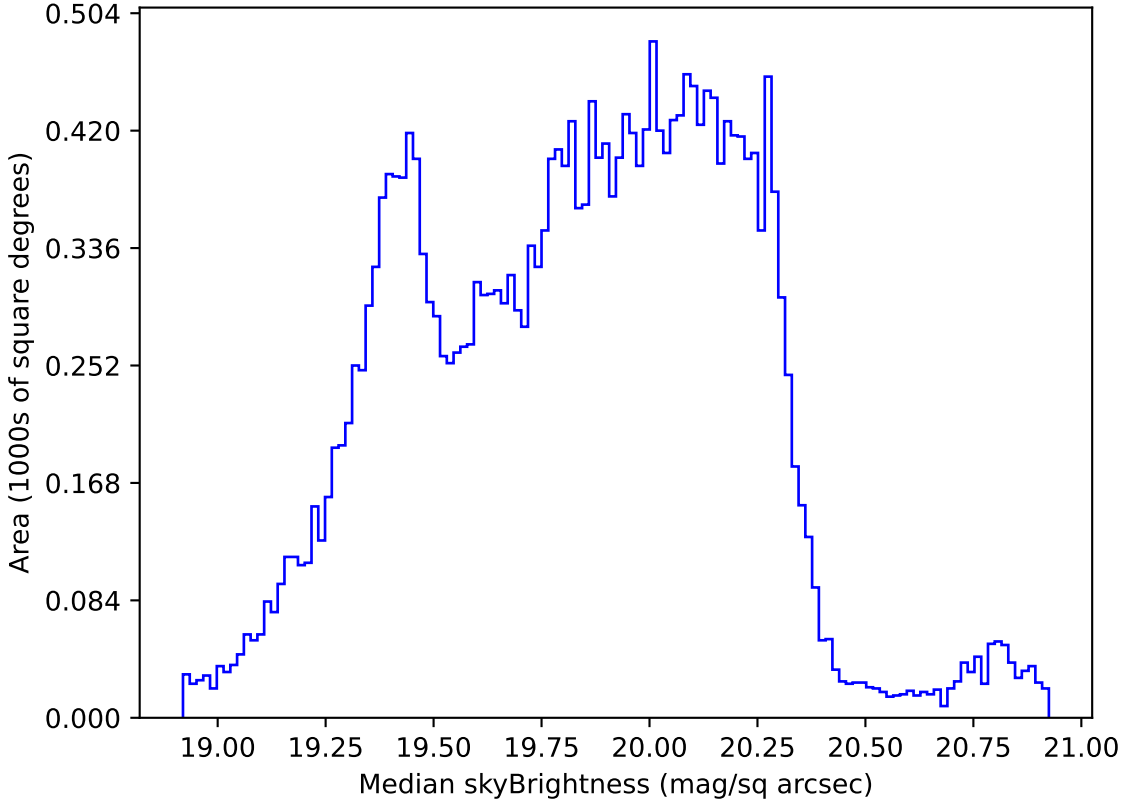
too_ignore_100_4v3.4_10yrs Yr 1 all bands: Median skyBrightness
