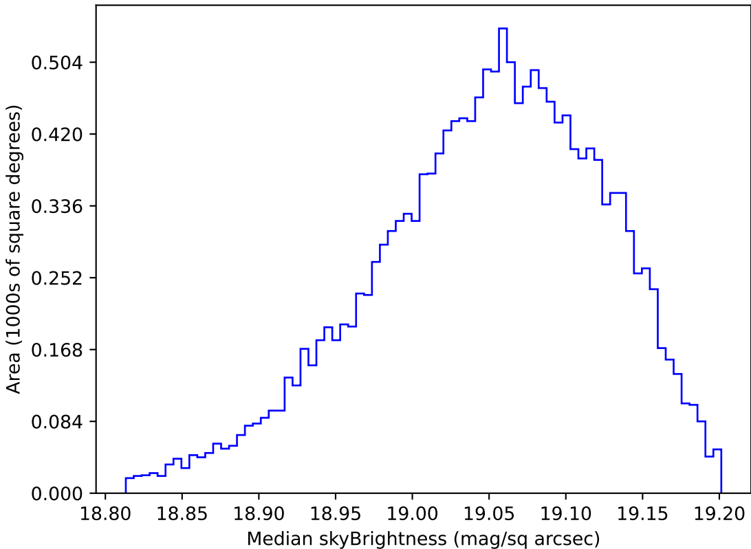
too_ignore_100_4v3.4_10yrs WFD z band: Median skyBrightness
