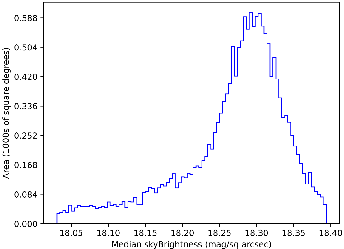
too_ignore_100_4v3.4_10yrs WFD y band: Median skyBrightness
