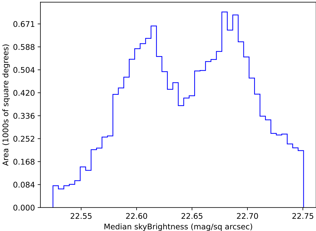
too_ignore_100_4v3.4_10yrs WFD u band: Median skyBrightness
