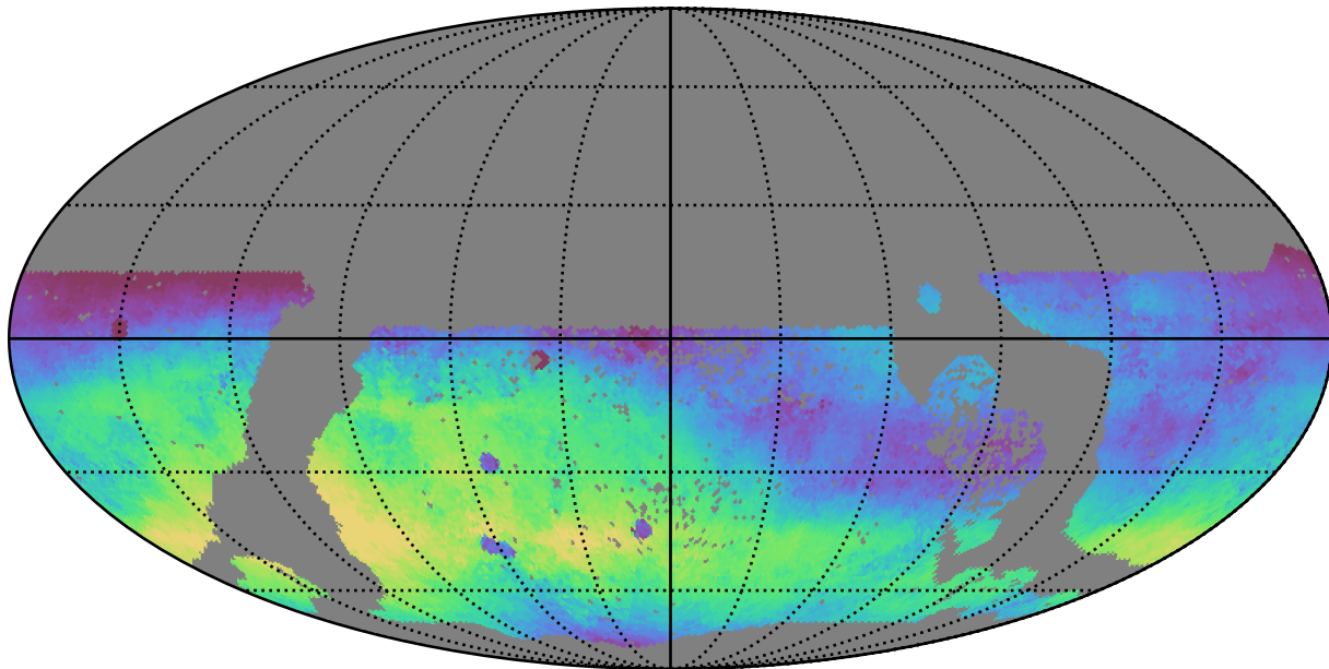
too_ignore_100_4v3.4_10yrs WFD r band: Median skyBrightness
