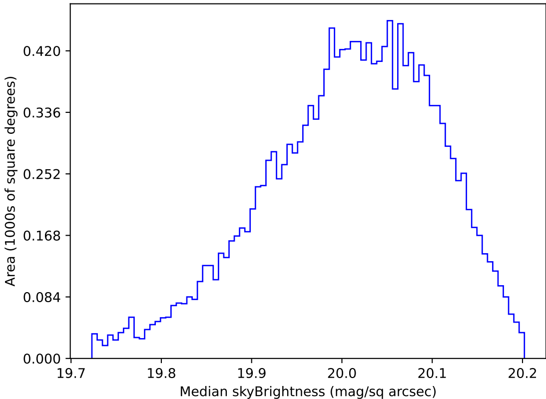
too_ignore_100_4v3.4_10yrs WFD i band: Median skyBrightness
