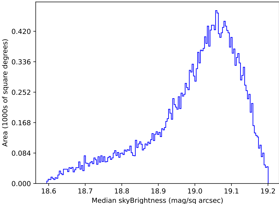
too_ignore_100_4v3.4_10yrs All sky z band: Median skyBrightness
