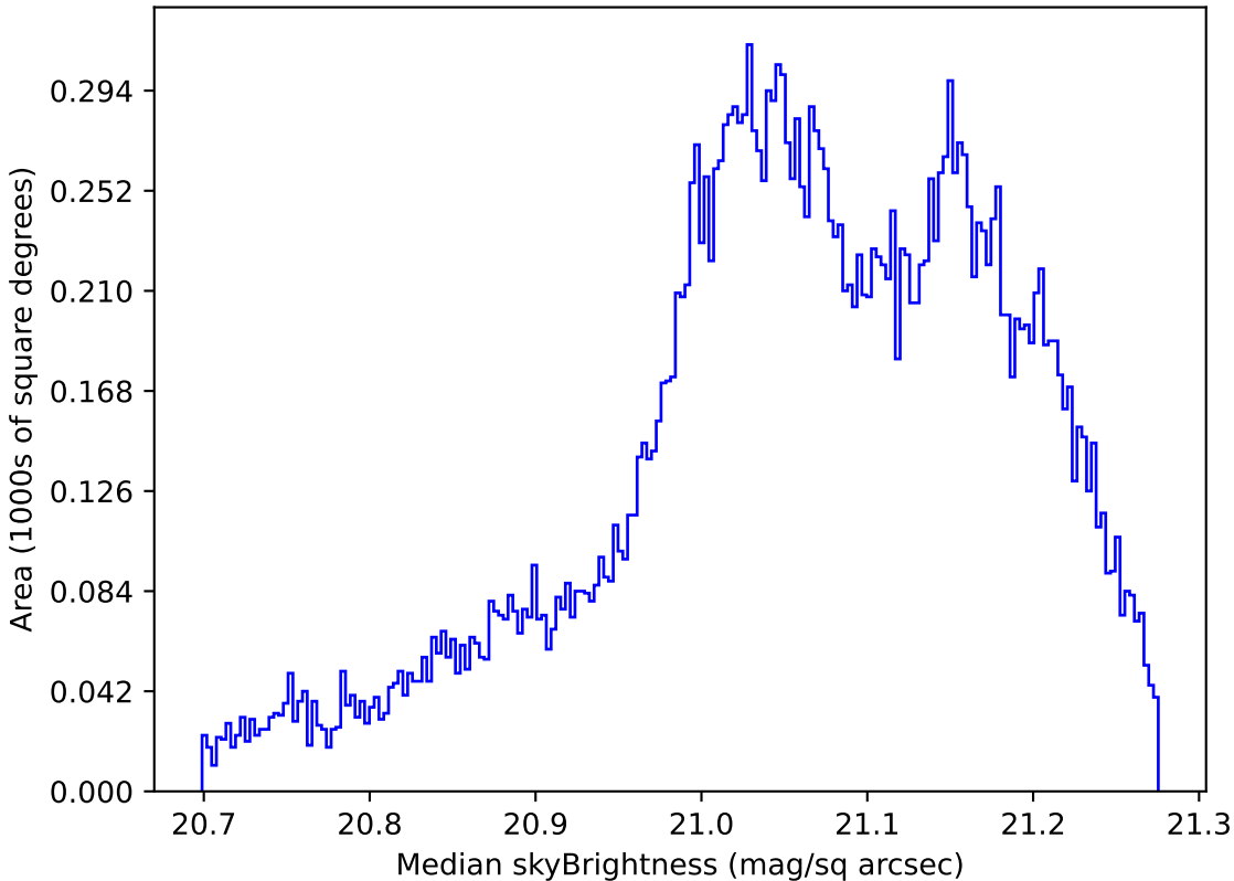
too_ignore_100_4v3.4_10yrs All sky r band: Median skyBrightness
