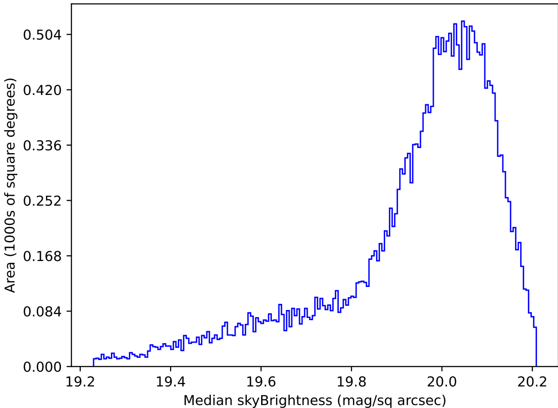
too_ignore_100_4v3.4_10yrs All sky i band: Median skyBrightness
