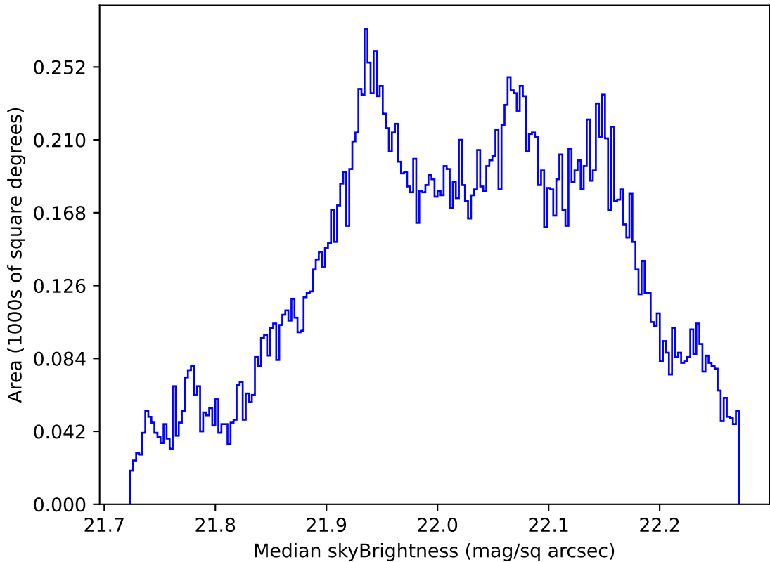
too_ignore_100_4v3.4_10yrs All sky g band: Median skyBrightness
