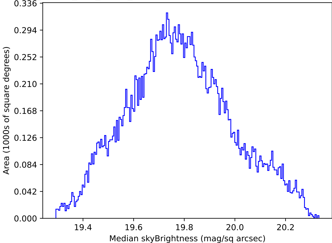
too_ignore_100_4v3.4_10yrs All sky all bands: Median skyBrightness
