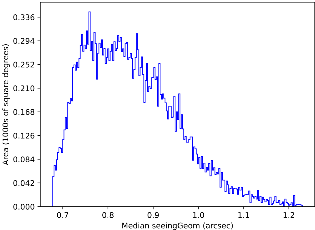
too_ignore_100_4v3.4_10yrs Yr 1 z band: Median seeingGeom
