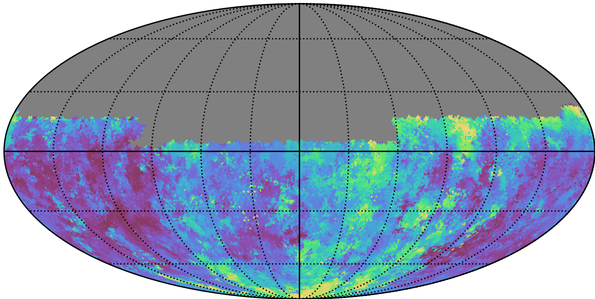
too_ignore_100_4v3.4_10yrs Yr 1 u band: Median seeingGeom
