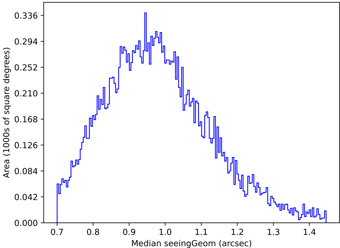
too_ignore_100_4v3.4_10yrs Yr 1 u band: Median seeingGeom
