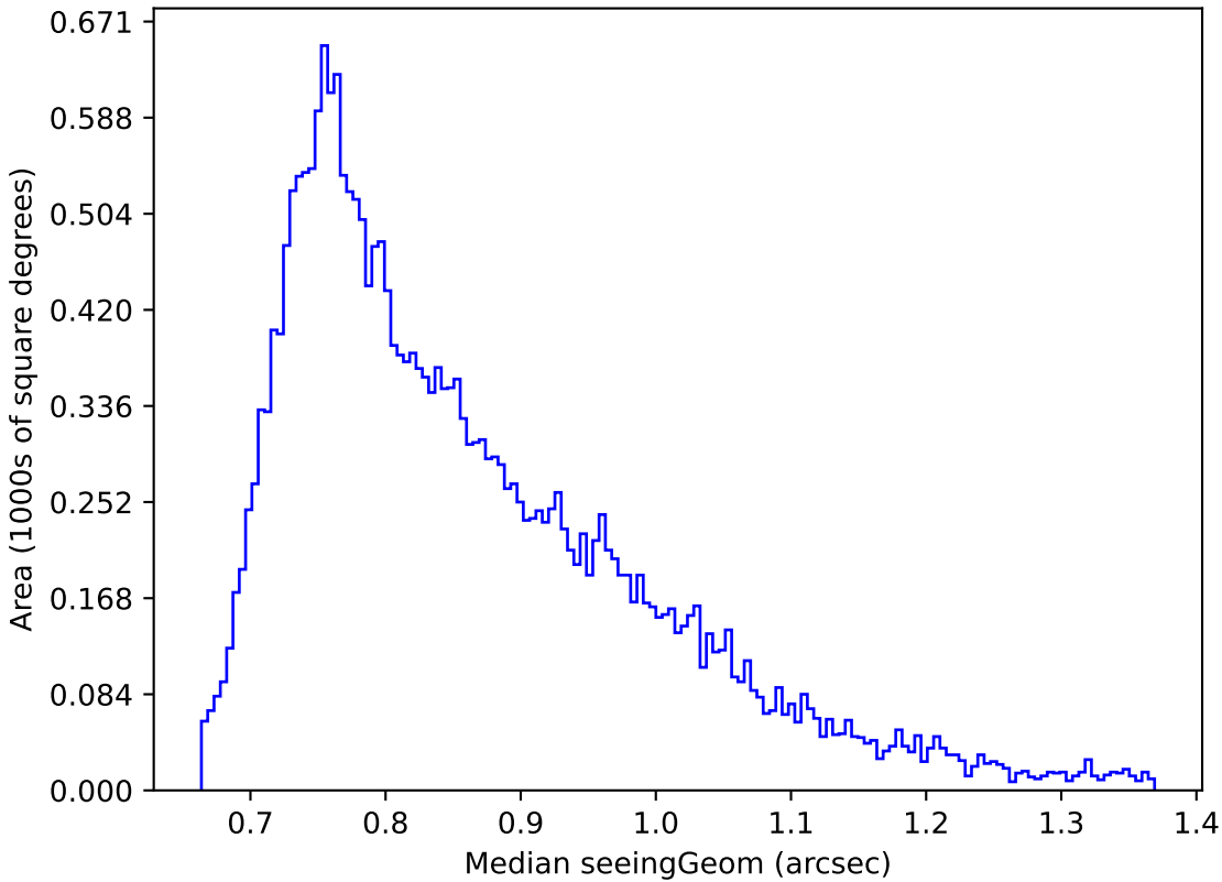
too_ignore_100_4v3.4_10yrs Yr 1 r band: Median seeingGeom
