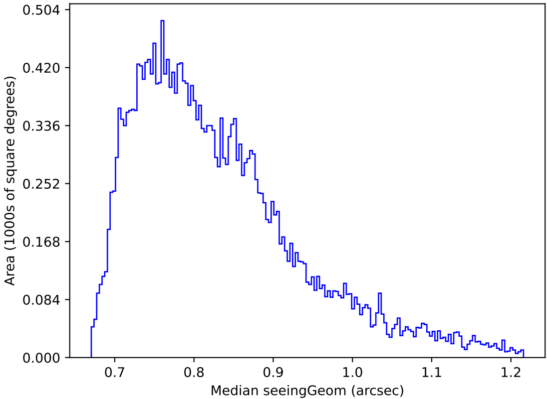
too_ignore_100_4v3.4_10yrs Yr 1 i band: Median seeingGeom
