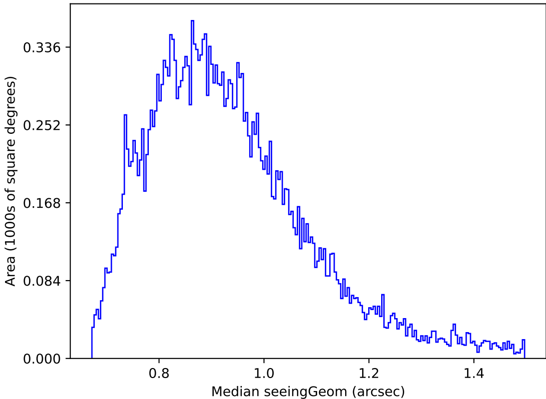
too_ignore_100_4v3.4_10yrs Yr 1 g band: Median seeingGeom
