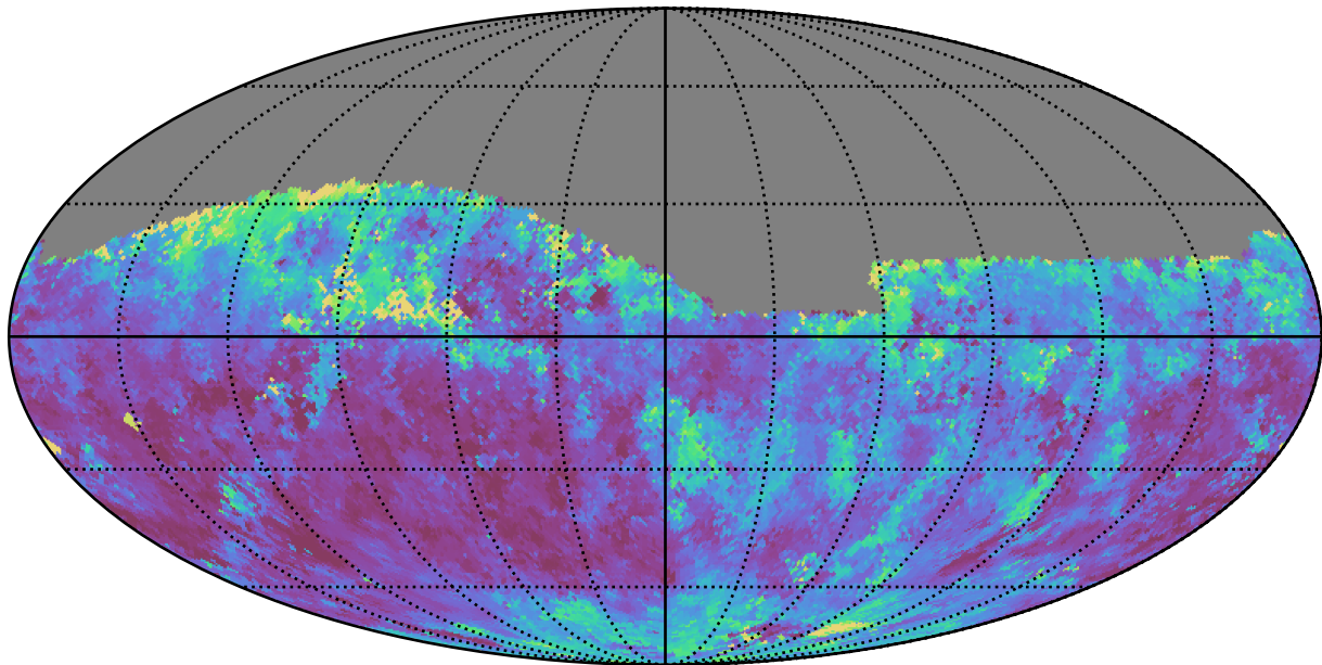
too_ignore_100_4v3.4_10yrs Yr 1 z band: Median seeingEff
