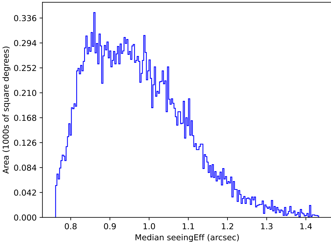
too_ignore_100_4v3.4_10yrs Yr 1 z band: Median seeingEff
