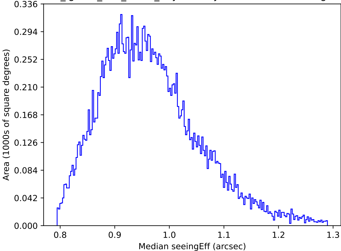
too_ignore_100_4v3.4_10yrs Yr 1 y band: Median seeingEff
