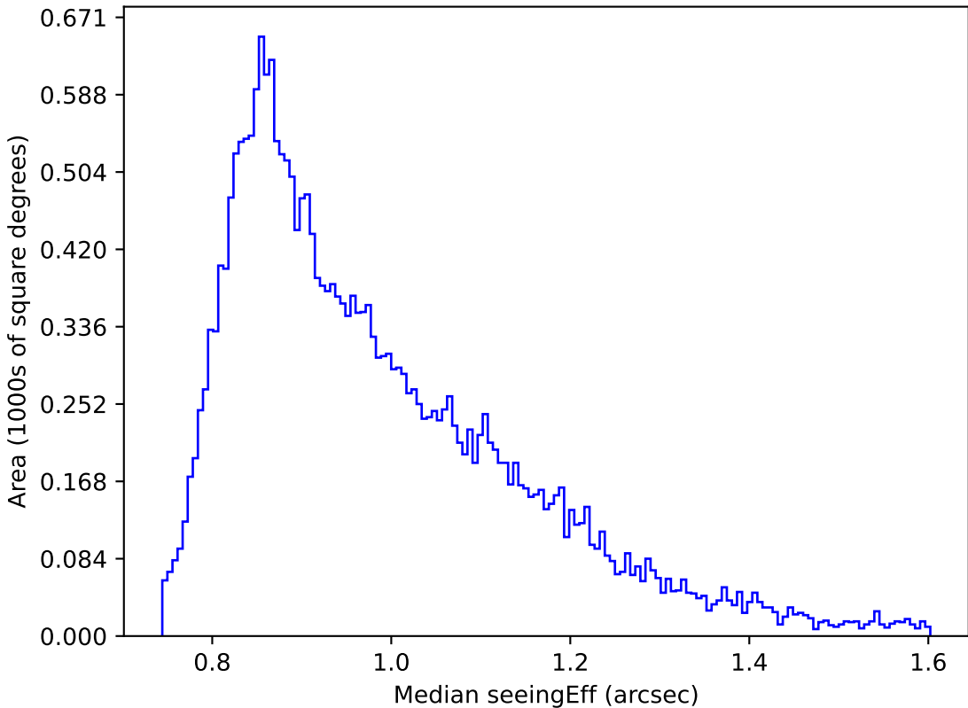
too_ignore_100_4v3.4_10yrs Yr 1 r band: Median seeingEff
