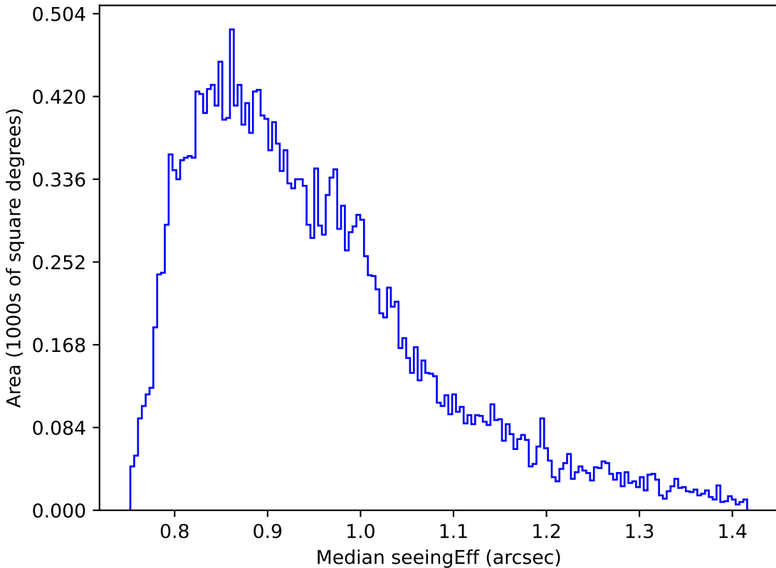
too_ignore_100_4v3.4_10yrs Yr 1 i band: Median seeingEff
