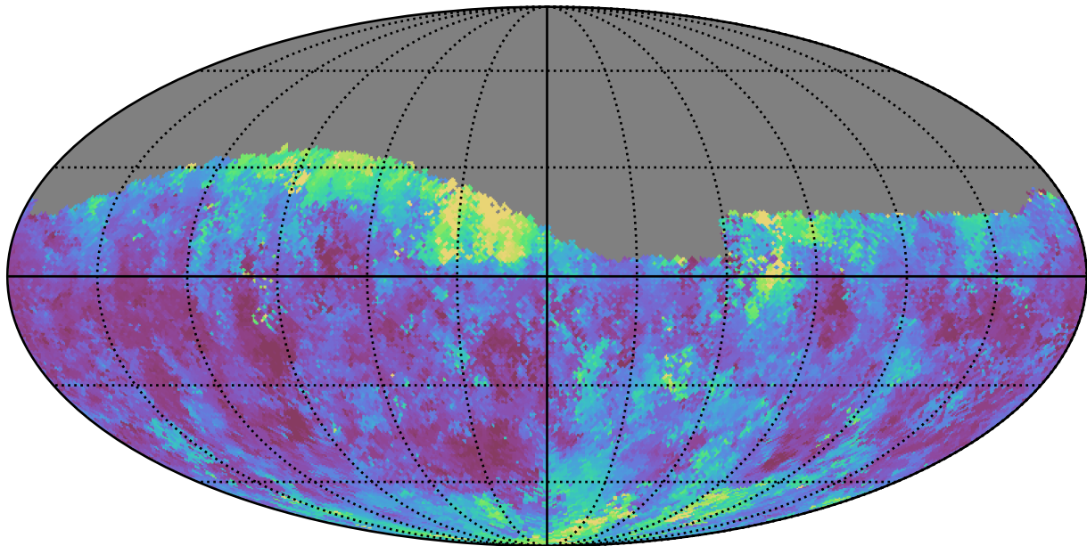
too_ignore_100_4v3.4_10yrs Yr 1 g band: Median seeingEff
