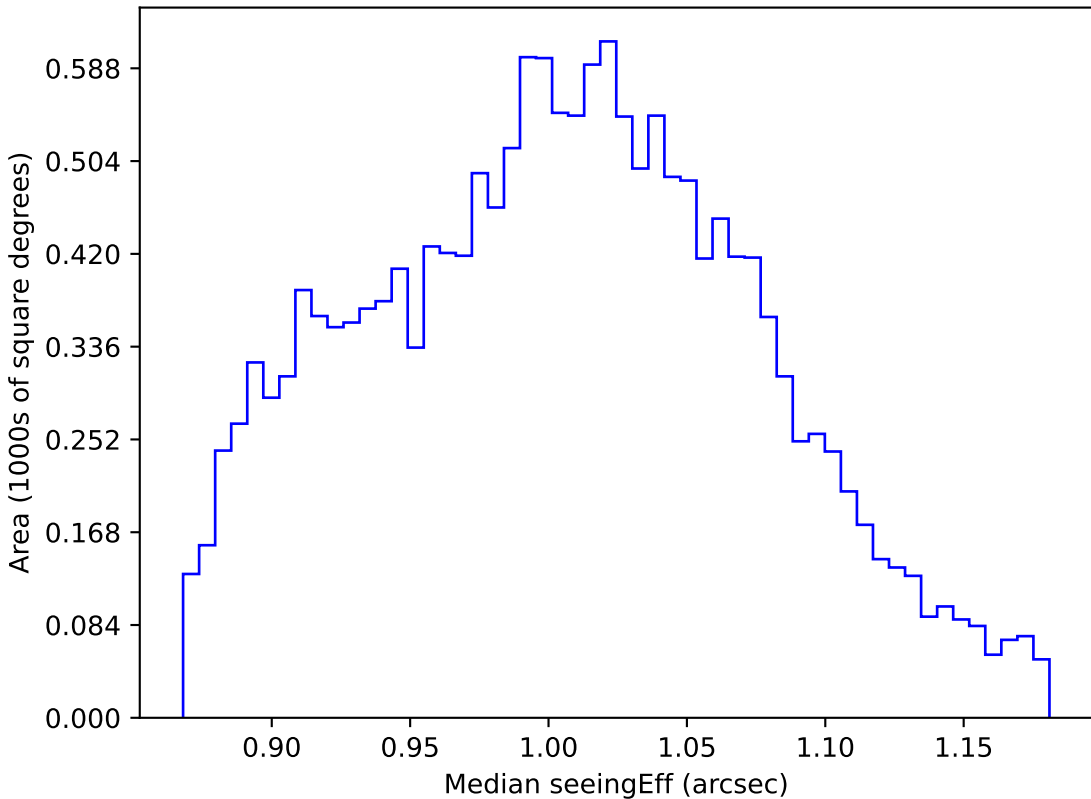
too_ignore_100_4v3.4_10yrs WFD z band: Median seeingEff
