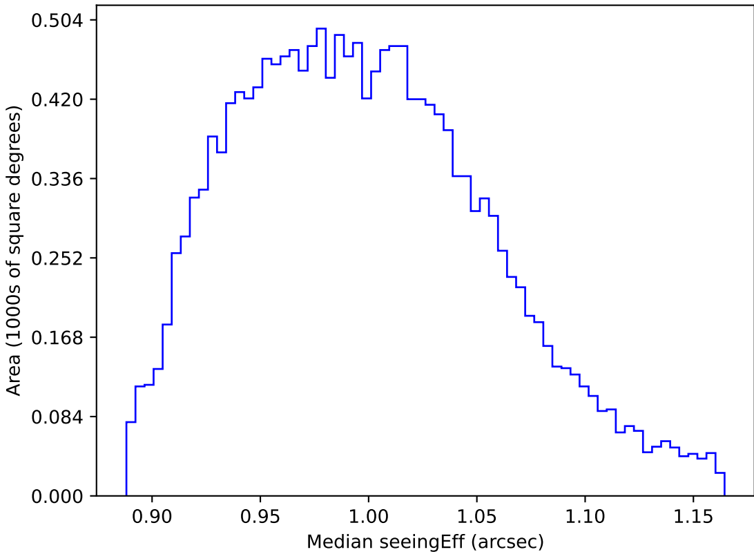
too_ignore_100_4v3.4_10yrs WFD y band: Median seeingEff
